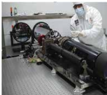
MCNS faculty working in a class 100 clean room at ISRO Bangalore: developing SUIT onboard Aditya-L1
