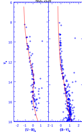
Figure 6. V_o/(U-B)_o and V_o/(B-V)_o CMD of stars lying within the cluster region of the cluster NGC 2129. Solid line is the Schmidt-Kaler (1982) shifted by distance modulus of 11.65 mag.
