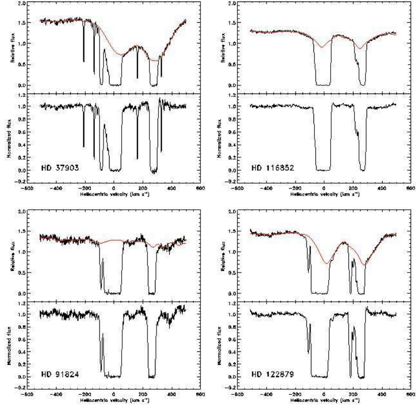
Figure 1. The observed stellar spectra are shown with interstellar line absorption from CII in velocity space. The stellar spectrum from the UVBLUE models is shown as a red line in each of the upper plates and is divided out in the bottom plates which are then used to derive the interstellar absorption.
