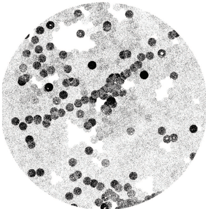
Figure 2. The density over the North Galactic Pole of stars with both GALEX and SDSS observations is shown. the bright regions are deep observations with fainter stars and thus a higher stellar density while the others are observations of as little as 100 s taken as part of the all-sky survey.
